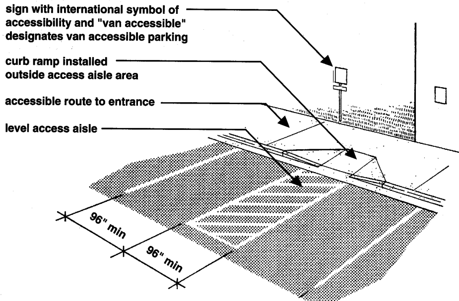
Diagram of Van Accessible Parking Space Elements
